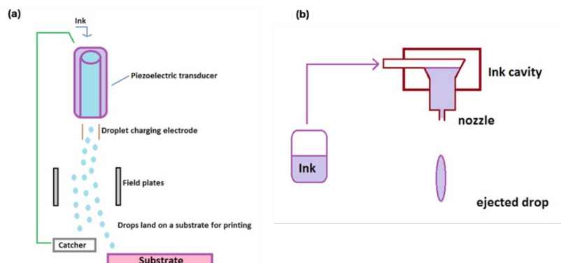
Fig. 9. Schematic diagram of a) continuous inkjet printer, b) drop-on-demand print head.
