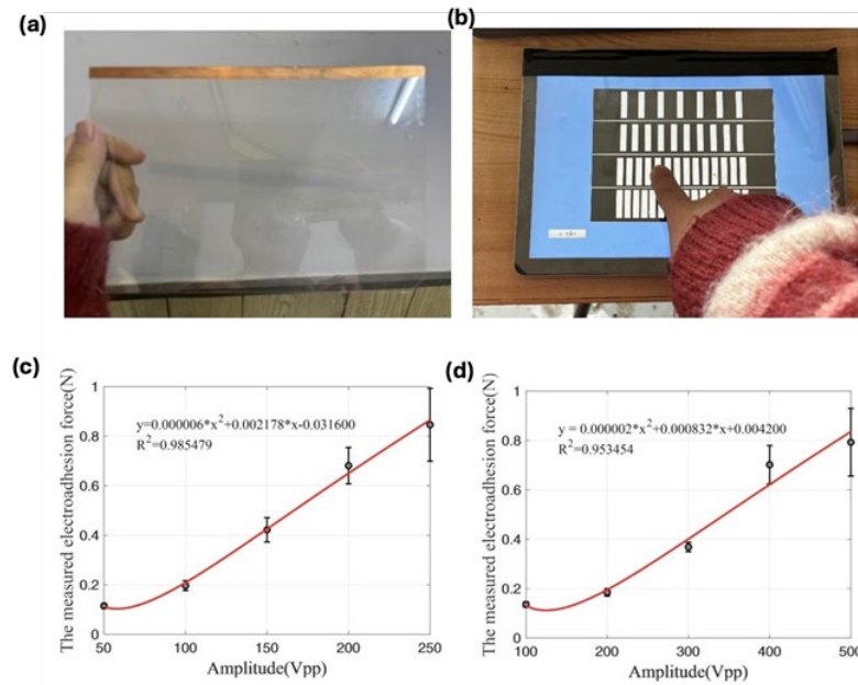
Fig. 3. (a) ATO panel and (b) integrated prototype, measured electro-adhesion forces of the two panels (c) 3M panel and (d) ATO panel (Z. Sun et al., 2024).
