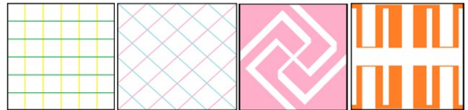
Fig. 1. Some electrode patterns for projected capacitive touch panel sensors. The name of the pattern from the left side to the right side is grid, diamond, interleaved, and angled cross pattern, respectively.
