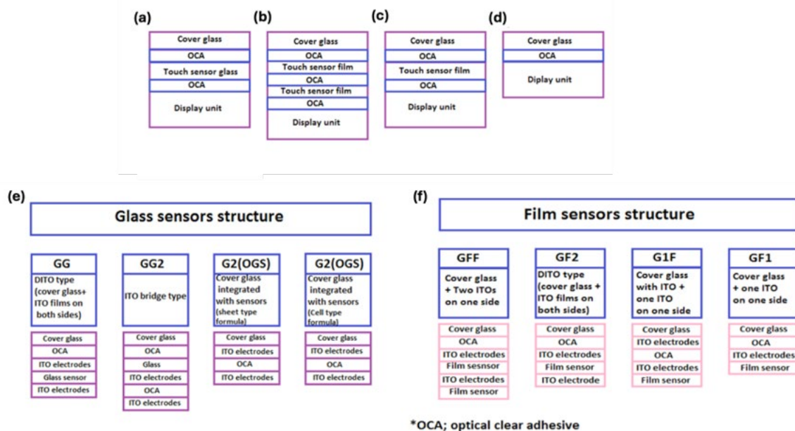
Fig. 4. (a-d) Projected capacitive touch panel structures, (e) glass sensor type, (f) film sensor type.
