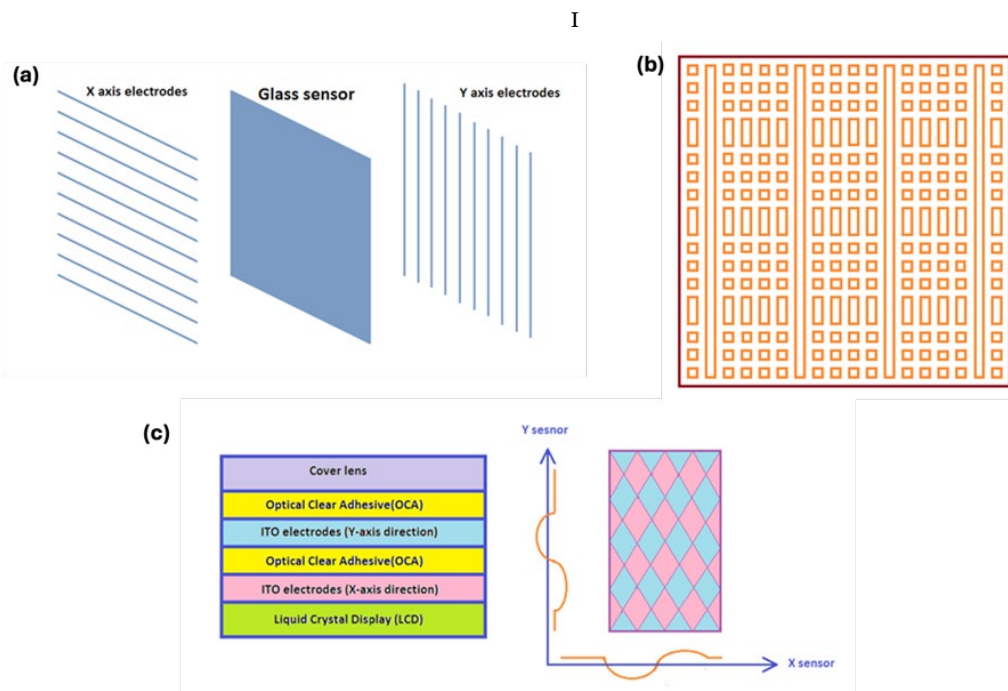
Fig. 5. a) iPhone pattern for touch panel conductor, b) Manhattan structure for electrode patterning in capacitive touch panels, c) The simple structure of projected capacitive touch panels.
