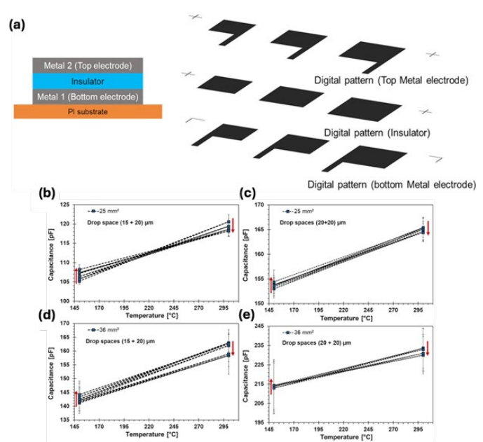
Fig. 10. a) Illustration of MIM device architecture on PI substrate with digital images showing printed structures with varying active areas. Graphs (b–e) depict capacitance changes during thermal cycles (150–300 °C) for 25 mm 2 and 36 mm 2 MIM devices with varying insulator thickness. Reprinted with permission (Mitra et al., 2024). Copyright 2024, Wiley.
