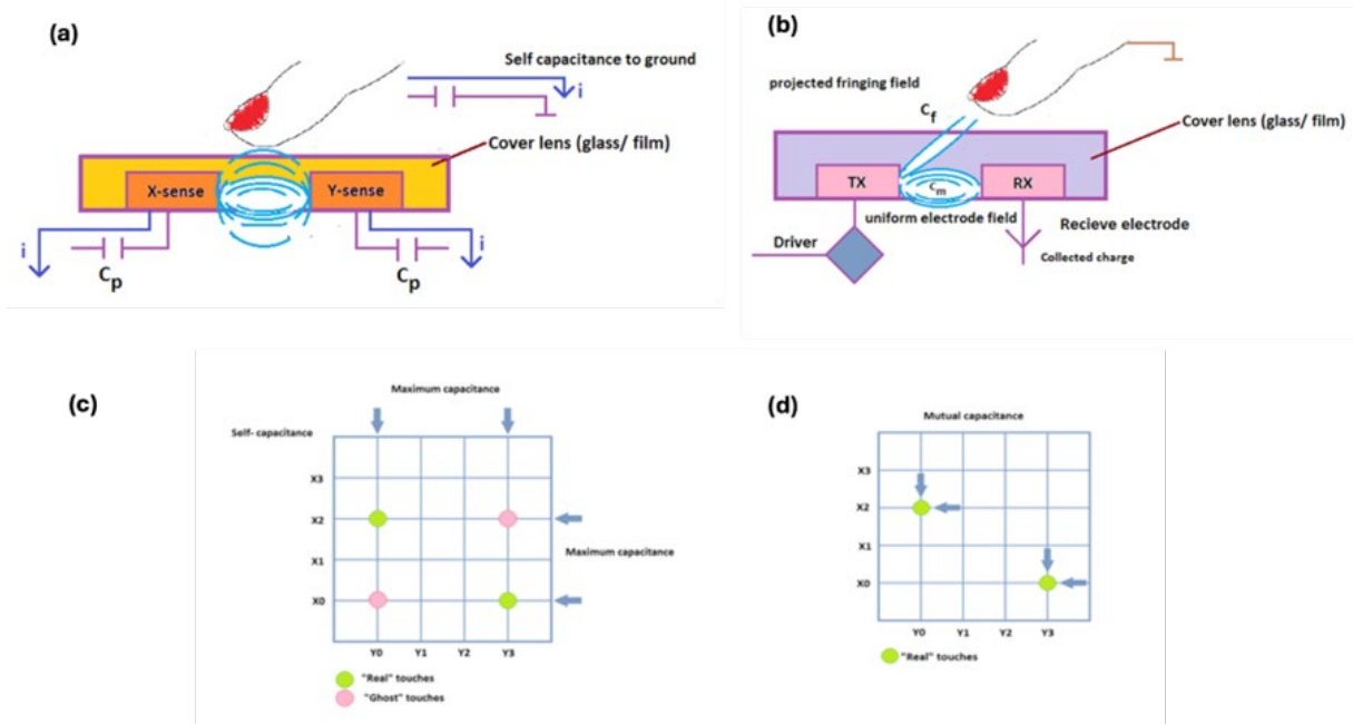
Fig. 2. (a and c) Self-capacitive and (b and d) mutual-capacitive sensing method.
