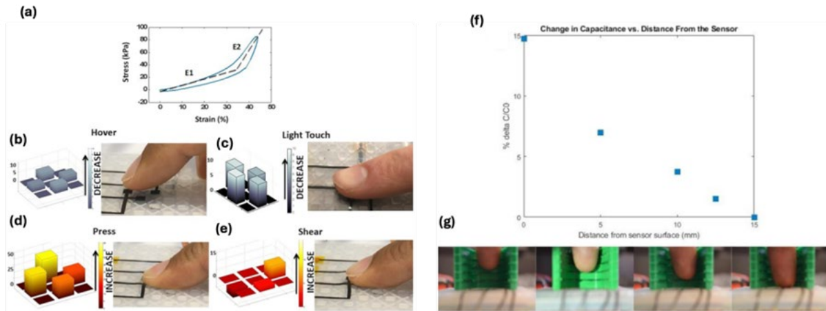
Fig. 6. Response of the sensor to various stimuli. (a) Non-linear elastic response (b) Hovering finger. response (c) Light touch response. (d) Pressure response. (e) Shear. response. Proximity characterization of approaching objects: (f) Taxel capacitive response with a baseline capacitance at 15 mm distance. (g) Finger approaching guide. Reprinted with permission (Sarwar et al., 2023). Copyright 2023, Springer Nature.
