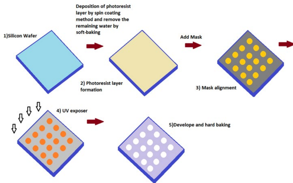
Fig. 7. Lithography electrode patterning process including substrate cleaning, barrier and photoresist layer formation, soft-baking, mask alignment, exposure, development, and hard-baking.
