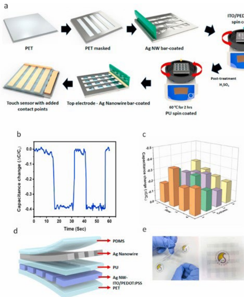
Fig. 8. The optoelectronic properties of the capacitive touch panel include a) fabrication process schematic, b) capacitance change per pixel, c) capacitance change for 16 pixels (10×10 cm), d) layer structure, and e) photograph of the flexible device (Raman et al., 2021).
